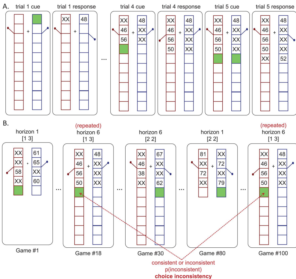
Fig 1. Schematic of the experiment. (A) Dynamics of an example horizon 6 game. Here the first four trials are forced trials in which participants are instructed which option to play. After the forced trials, participants are free to choose between the two options for the remainder of the game. (B) Example repeated games over the course of the experiment. On average, participants play more than 150 such games, with varying horizon (1 vs 6), uncertainty condition ([1 3] vs [2 2]) and observed rewards. In addition, all games are repeated (as Game 18 and 100 are here) such that participants will be faced with the exact same pattern of forced trials and exact same outcomes from those forced trials twice within each experiment. These repeated games allow us to compute the relative contribution of deterministic and random noise by analyzing the extent to which choices are consistent across the repeated games.
