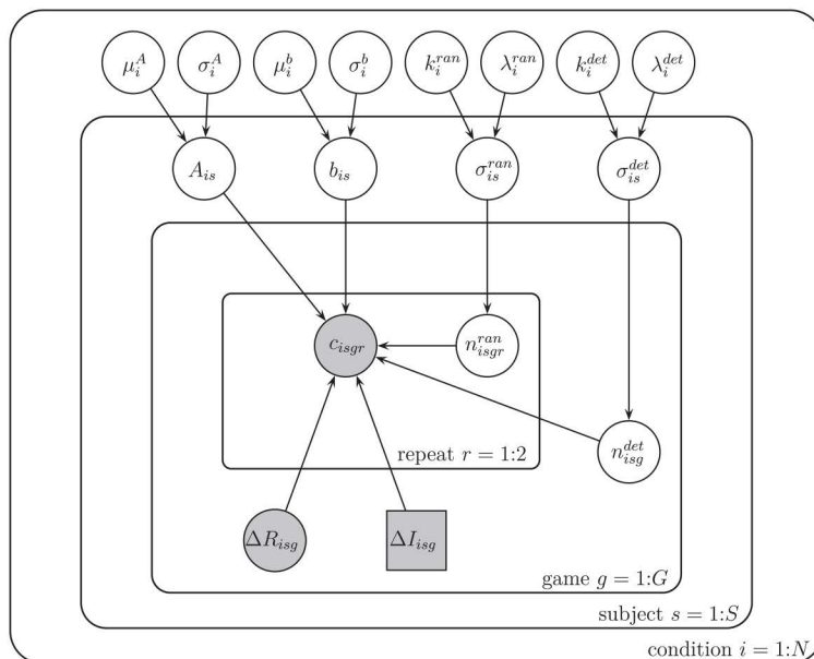
Fig 8. Schematic of the hierarchical Bayesian model using notation of [38].
